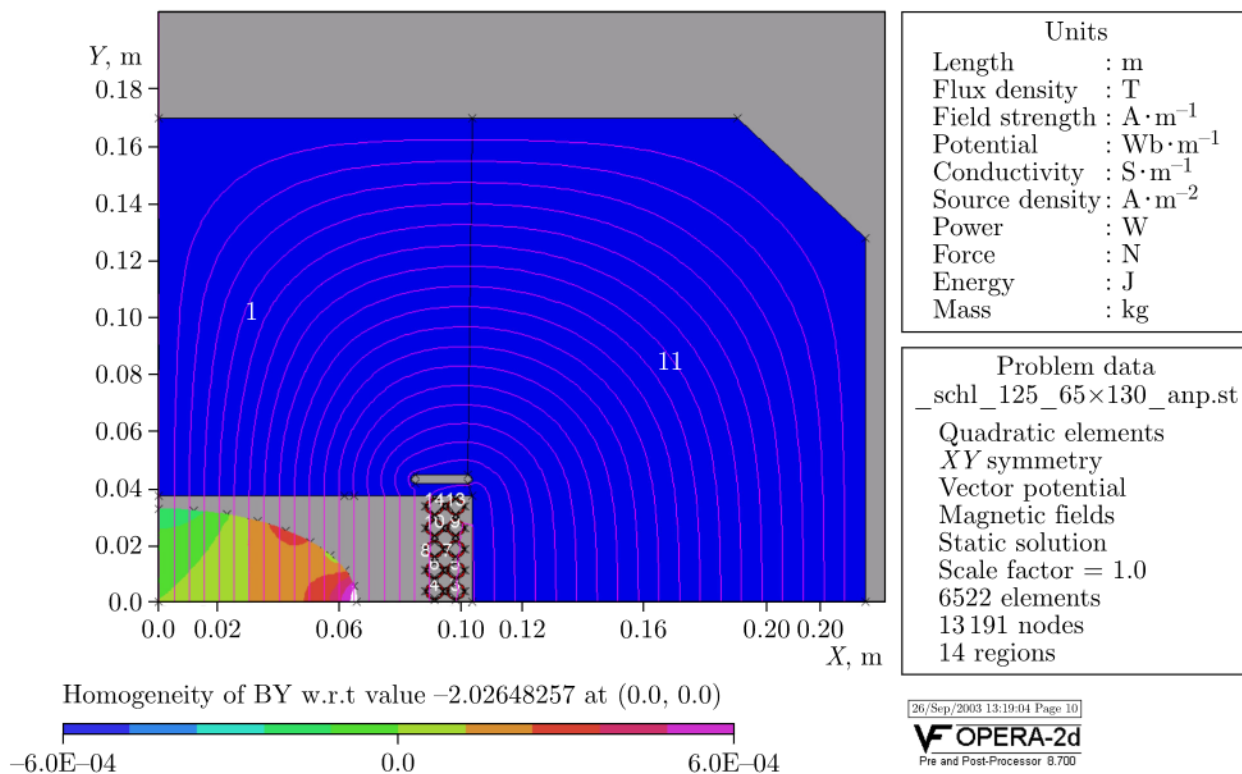
Figure 6. Magnetic field distribution in the model SIS100 magnet with negative shims.
