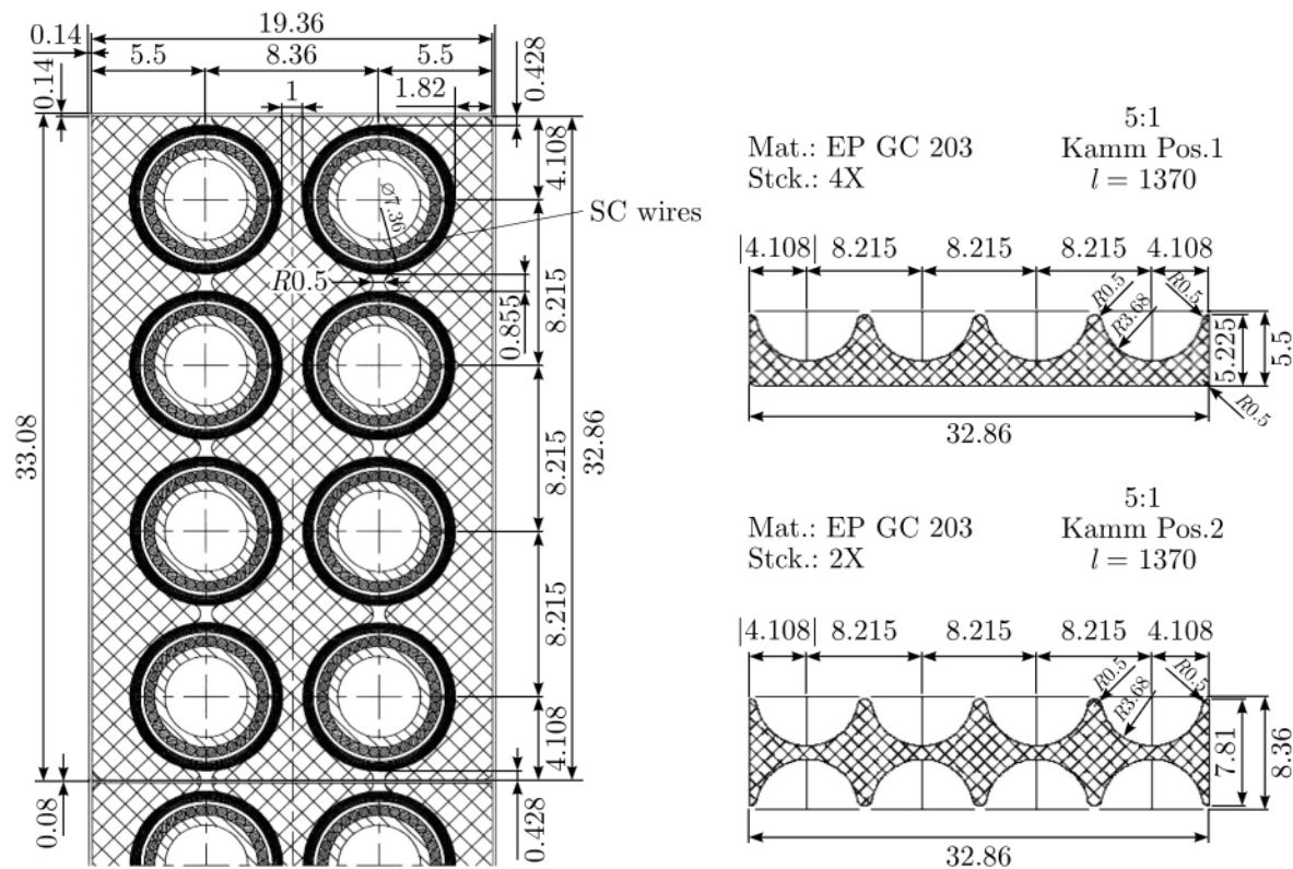
Figure 7. Coil support structure.
