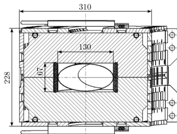
Figure 9. The dipole of the NICA Booster.
