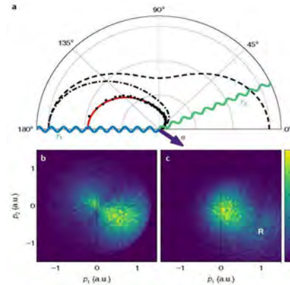
Scheme of ionization by Compton scattering at h\nu=2.1 keV
