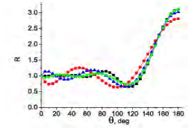
P.B. Kats, A.V. Kudravets, A.S. Rimashevskaya, O.O. Voskresenskaya // Radiation Physics and Chemistry 222 (2024) 111860
