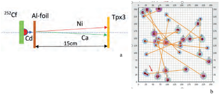
FIGURE 4. Schematical presentation of the tri-partition of the mother nucleus ^{252}\text{Cf} \rightarrow \text{Sn} + \text{Cd} \rightarrow \text{Ni} + \text{Ca} chosen as an example of the CCT and kinematics of the decay partners in the TDS-1 setup (a). Typical result of the data processing (b). The cluster 10 marked by the red arrow is presumably due to the CCT event, while the orange arrow connects this cluster with another one produced most likely by the Al ion knocked out from the foil by Cd-like fragment.
