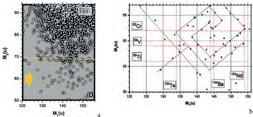
FIGURE 6. Correlation mass distribution of the FFs from ^{252}\text{Cf}(\text{sf}) obtained at the COMETA setup. Specific rhombic meander structure is marked by the arrow (a). The same structure in the larger scale (b). The meander vertexes coincide with known magic isotopes listed in boxes.
