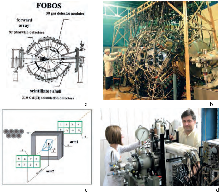
FIGURE 1. Design of the 4\text{-}\pi FOBOS spectrometer (a) and its overall view (b). Design of the COMETA setup (c). In the presented version it consists of two mosaics of eight PIN diodes each (4), microchannel-plates-based start-detector (2) with the ^{252}\text{Cf} source inside (1) and neutron belt consisting of 32 ^3\text{He} filled neutron counters (3). The overall view of the setup is shown in figure 1(d).
