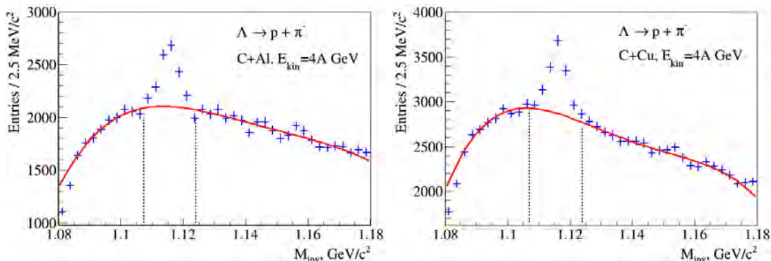
Signals \Lambda of hyperons in the spectra of invariant masses ( p, \pi^- ) measured in C+Al and C+Cu interactions.
