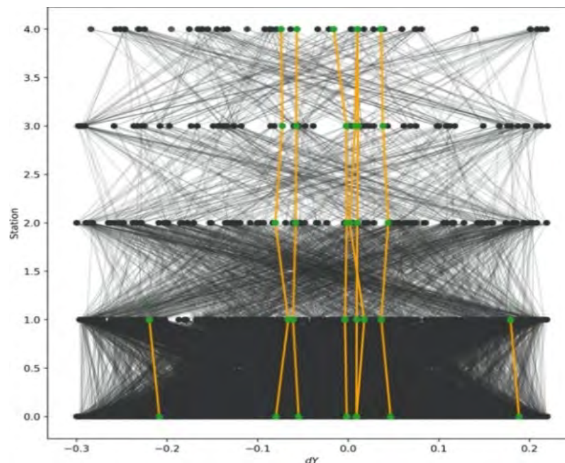
Graphical representation of C+C 4 GeV events of the BM@N experiment. Black nodes and edges correspond to fakes, green nodes and yellow edges correspond to found tracks.
