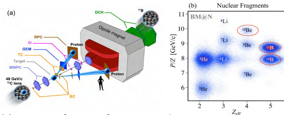
(a) BM@N configuration for SRC research.
